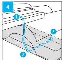
Innofix Clip Securing roof tiles to prevent wind-upliftment.
